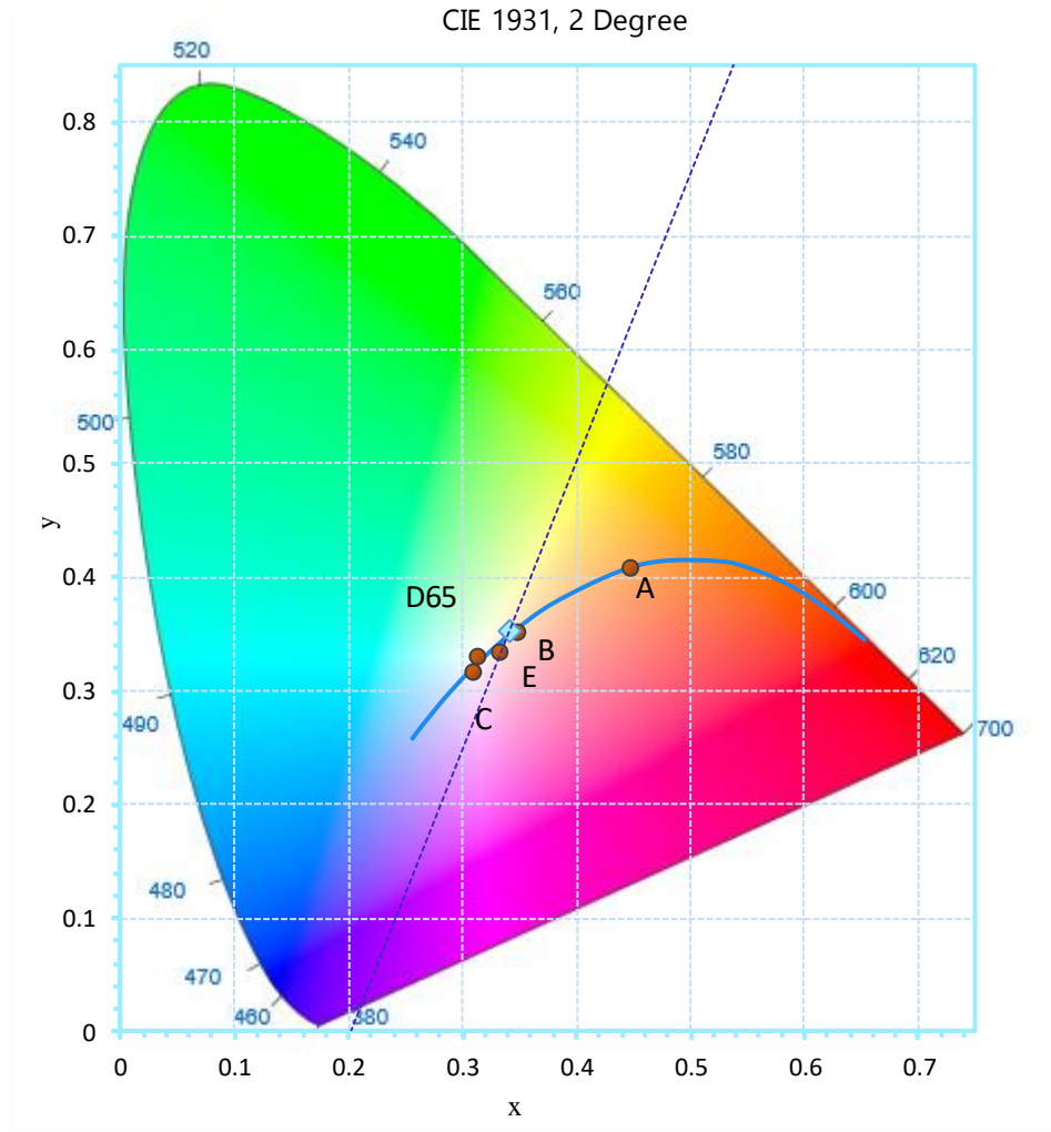
Chart 2. Chromaticity Diagram
